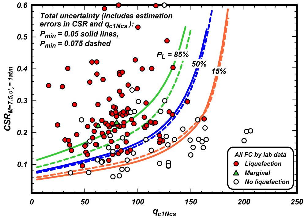
Figure 5.3. CRR_{M=7.5, \sigma'_v=1atm} versus q_{c1Ncs} for P_L = 15, 50 , and 85\% for all sands with FC based on laboratory test data, with inclusion of estimation errors in CRR_{M=7.5, \sigma'_v=1atm} and q_{c1Ncs} , and using P_{min} = 0.05 or 0.075 . Solutions for cases 5a and 5b from Tables 5.3 and 5.4
