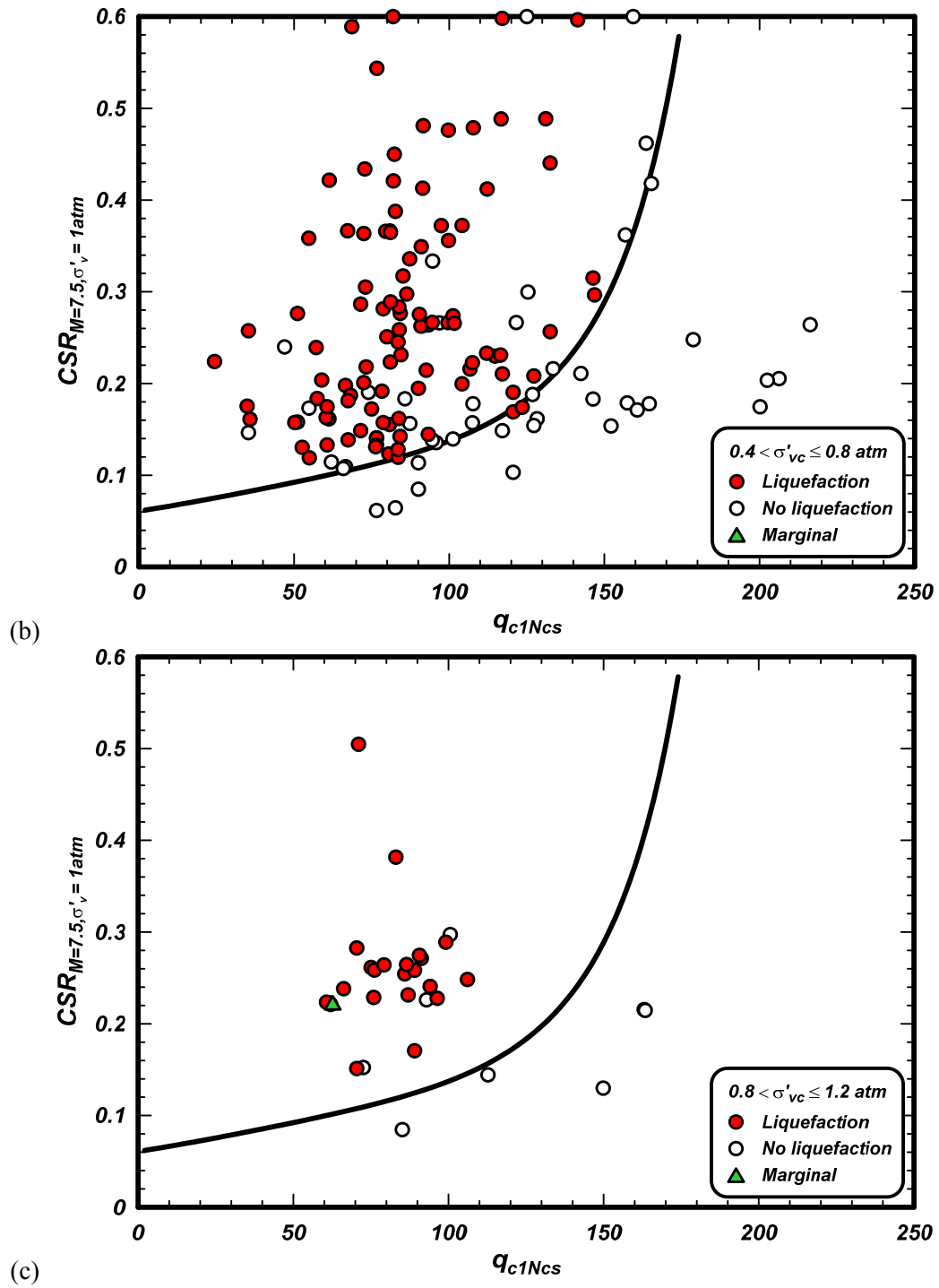
Figure 4.5b-c. Distribution of case history data with different effective overburden stresses and processed with the revised MSF relationship
