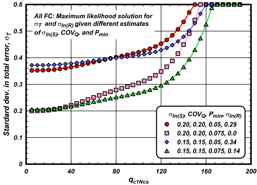
Figure 5.5. Standard deviation in the total error term ( \sigma_T ) and CRR relationship ( \sigma_{\ln(R)} ) from the maximum likelihood solution for different estimates of \sigma_{\ln(S)} and COV_Q in any FC sand. Solutions for cases 4a and 5a (Table 5.3) and 4b and 5b (Table 5.4)
