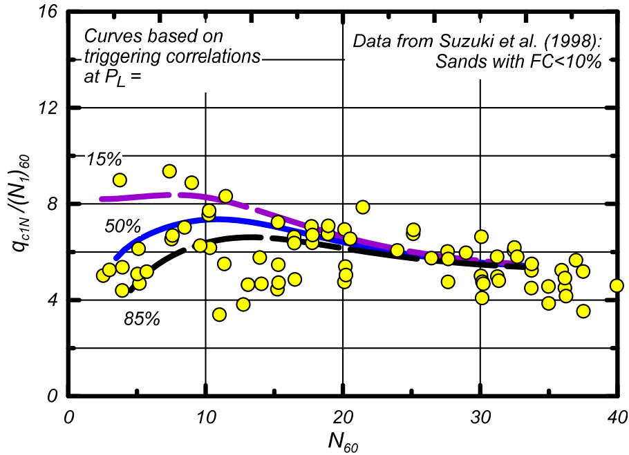
Figure 7.1. Ratio of q_{c1N}/N_{60} as a function of N_{60} in sands with FC \leq 10\% (data from Suzuki et al. 1998)
