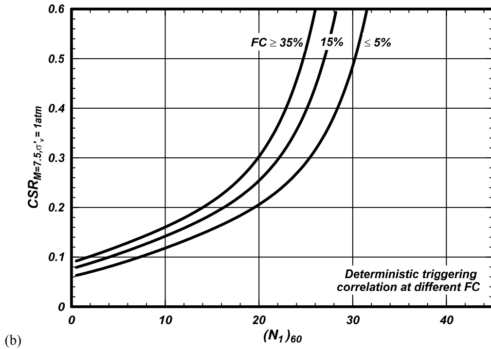
Figure 2.8. (a) Revised deterministic CPT-based triggering correlation and (b) the unchanged deterministic SPT-based triggering correlation for clean sands and for cohesionless soils having various values of FC.
