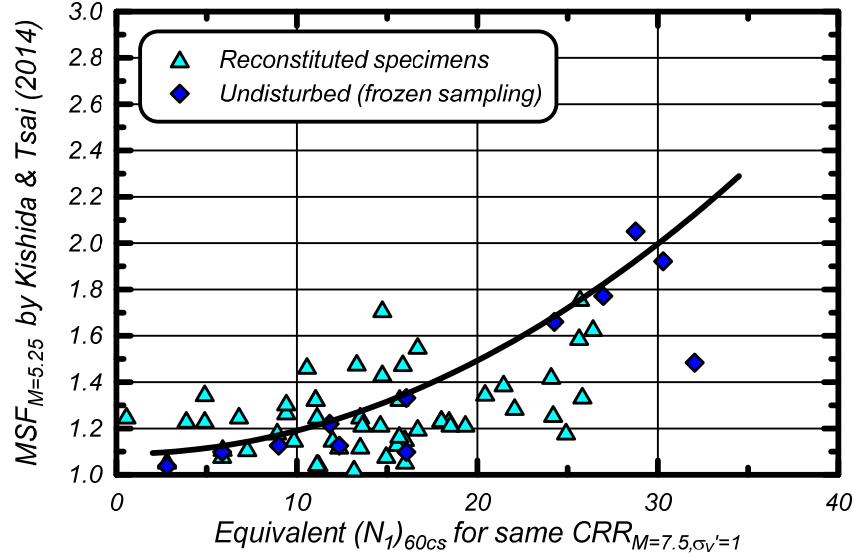
Figure A.22. Variation in MSF_{M=5.25} , computed using Kishida and Tsai's (2014) results, with equivalent (N_1)_{60cs} for cohesionless soils
