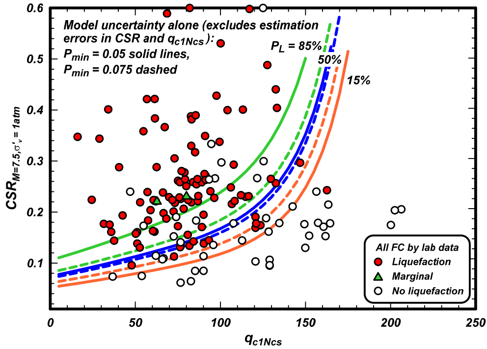
Figure 5.4. CRR_{M=7.5, \sigma'_v=1atm} versus q_{c1Ncs} for P_L = 15, 50 , and 85\% for all sands with FC based on laboratory test data, with model uncertainty alone (excluding estimation errors in CRR_{M=7.5, \sigma'_v=1atm} and q_{c1Ncs} ), and using P_{min} = 0.05 or 0.075 . Solutions for cases 5a and 5b from Tables 5.3 and 5.4
