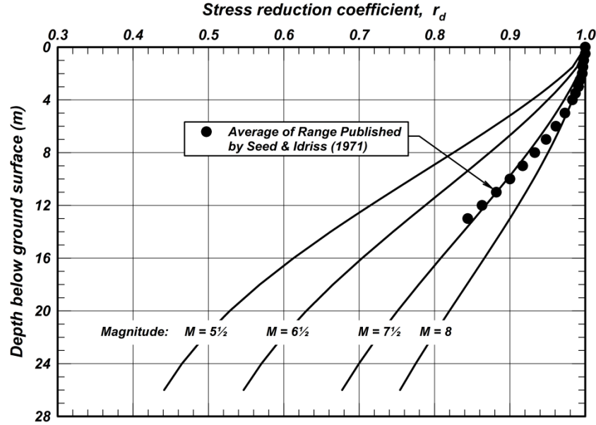
Figure 2.1. Shear stress reduction factor, r_d , relationship
