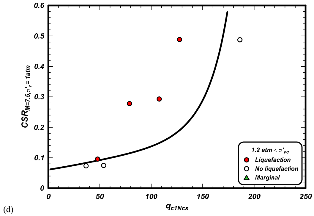
Figure 4.5d. Distribution of case history data with different effective overburden stresses and processed with the revised MSF relationship
