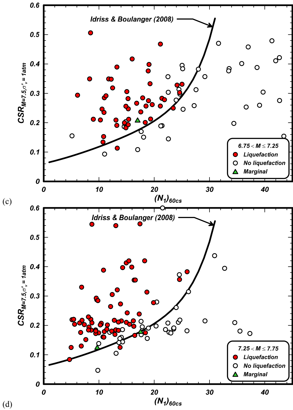
Figure 6.4c-d. Distribution of case history data with different earthquake magnitudes and processed with the revised MSF relationship
