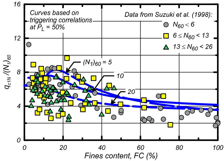
Figure 7.2. Ratio of q_{c1N}/(N_1)_{60} as a function of FC (data from Suzuki et al. 1998)
