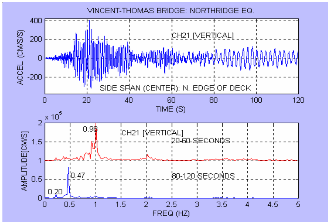
Figure 1. The recorded acceleration time-history of vertical motions at center of side-span exhibited the largest peak acceleration during the 1994 Northridge earthquake. This record also shows that the frequency of the bridge changed drastically (to 0.47 Hz) during the last 40 seconds of the record as compared to the 20-60 second band (0.98 Hz).
