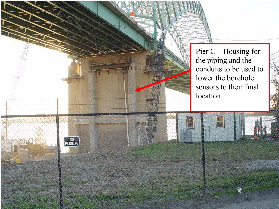
Figure 8. The location where the piping and conduits are housed for the installation of the downhole instruments at Pier C.
