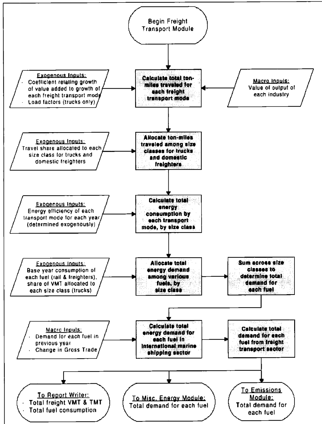
Figure 2.1 The Freight Module in the DOE's NEMS Model
