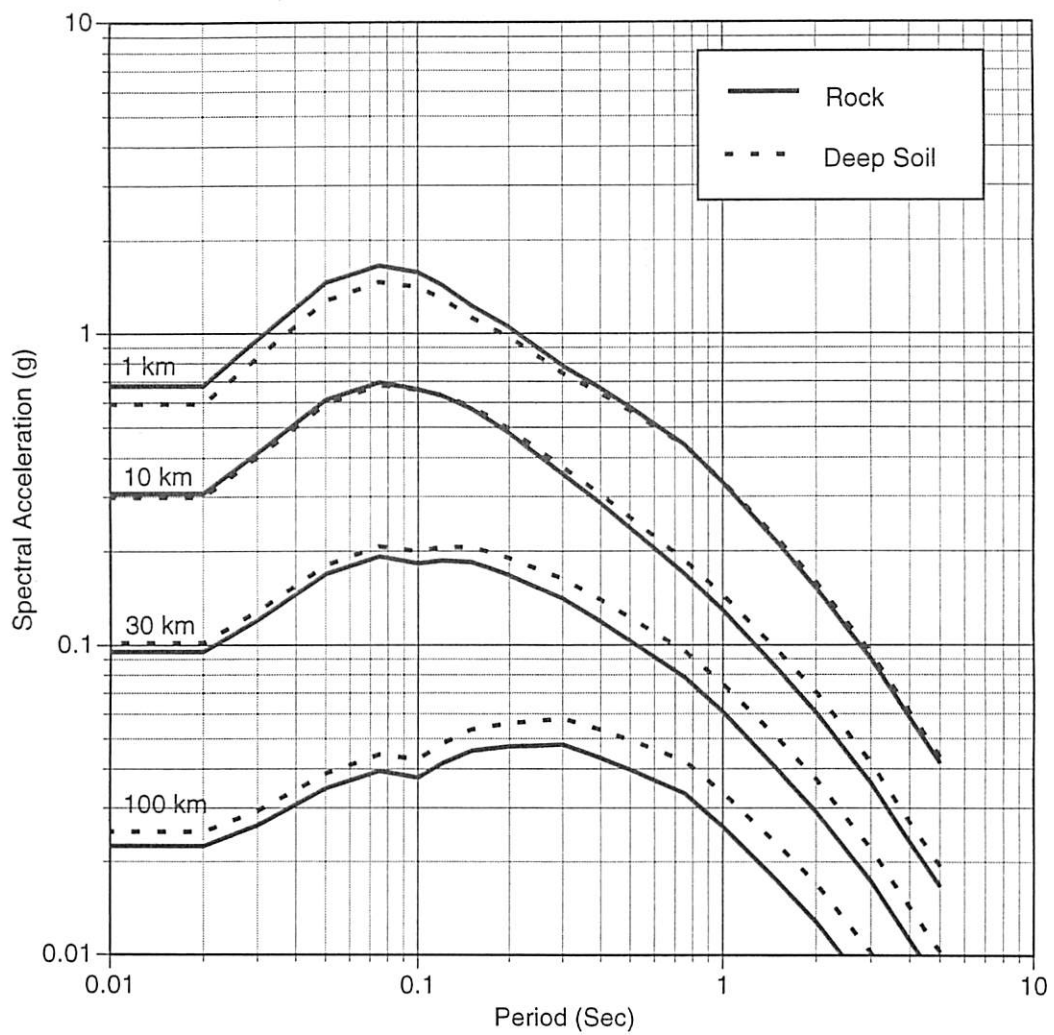
▲ Figure 10. Median model predictions for magnitude 7.0 strike-slip earthquakes for the vertical component.
