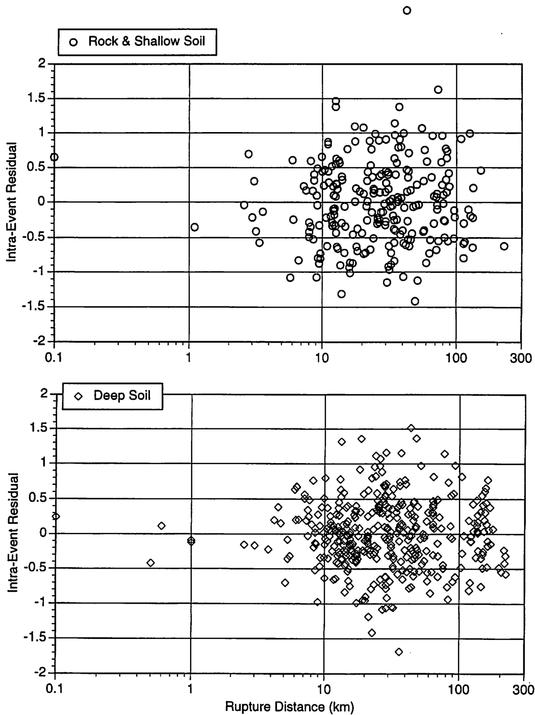
▲ Figure 4b. Distance dependence of the intra-event residuals for 0.3 second period for the horizontal component.
