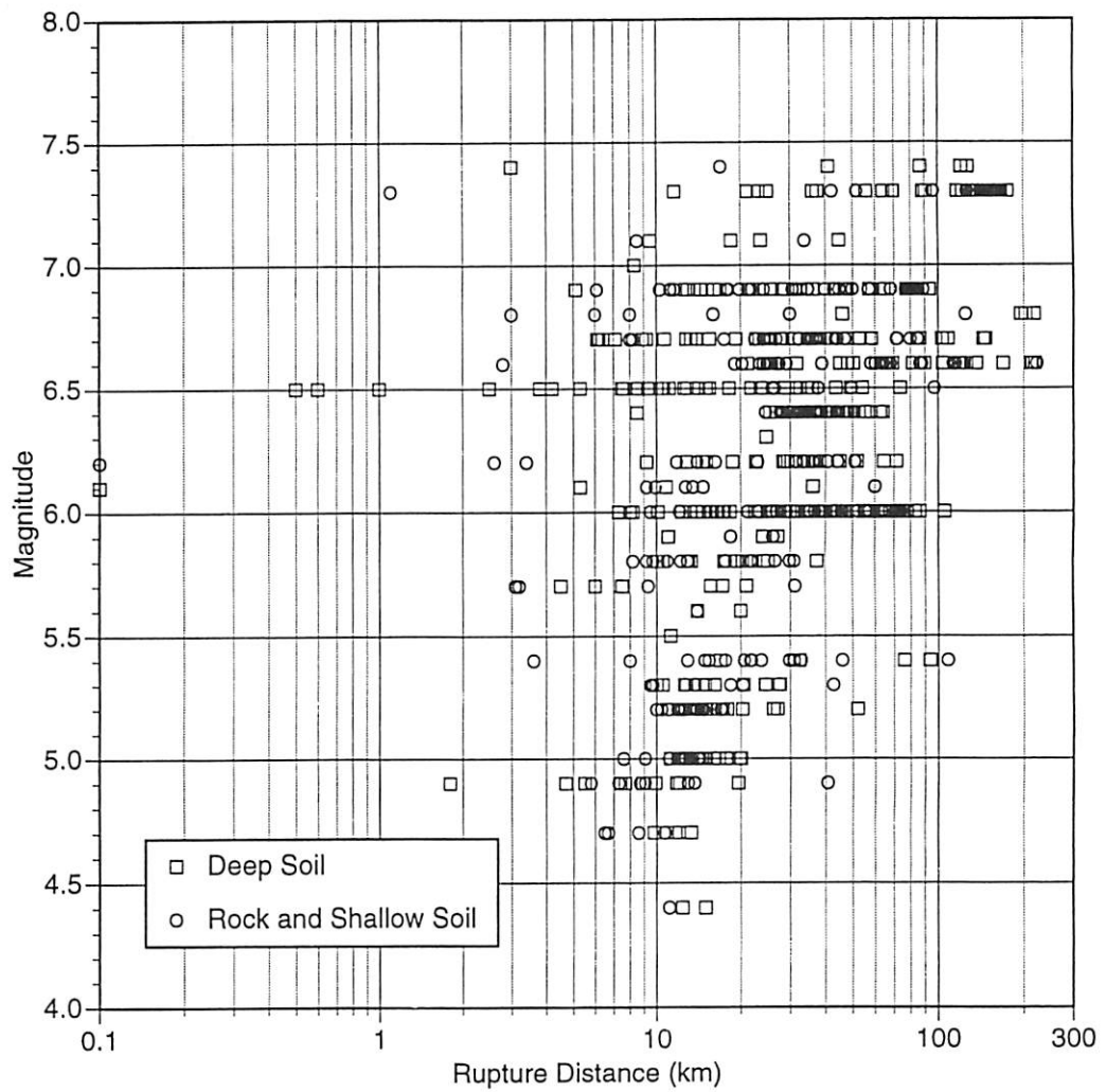
▲ Figure 2c. Distribution of data for 0.2 second period for the horizontal component.
