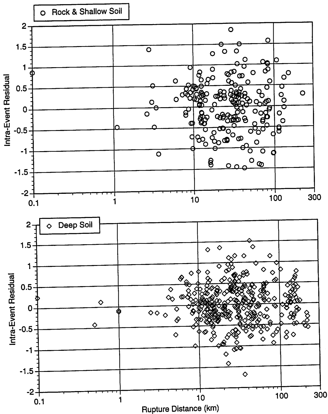
▲ Figure 4a. Distance dependence of the intra-event residuals for 1.0 second period for the horizontal component.
