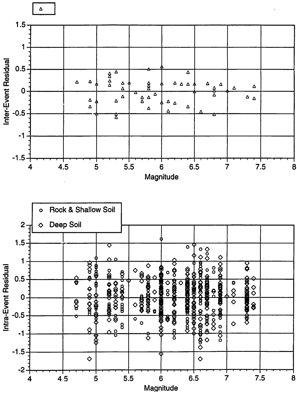
▲ Figure 5c. Magnitude dependence of the inter-event residuals (top) and the intra-event residuals (bottom) for 0.1 second period for the horizontal component.
