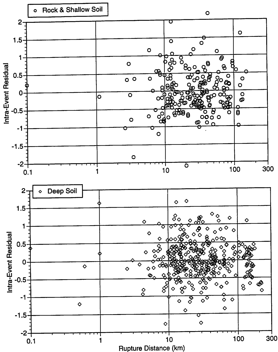
▲ Figure 6c. Distance dependence of the intra-event residuals for 0.1 second period for the vertical component.
