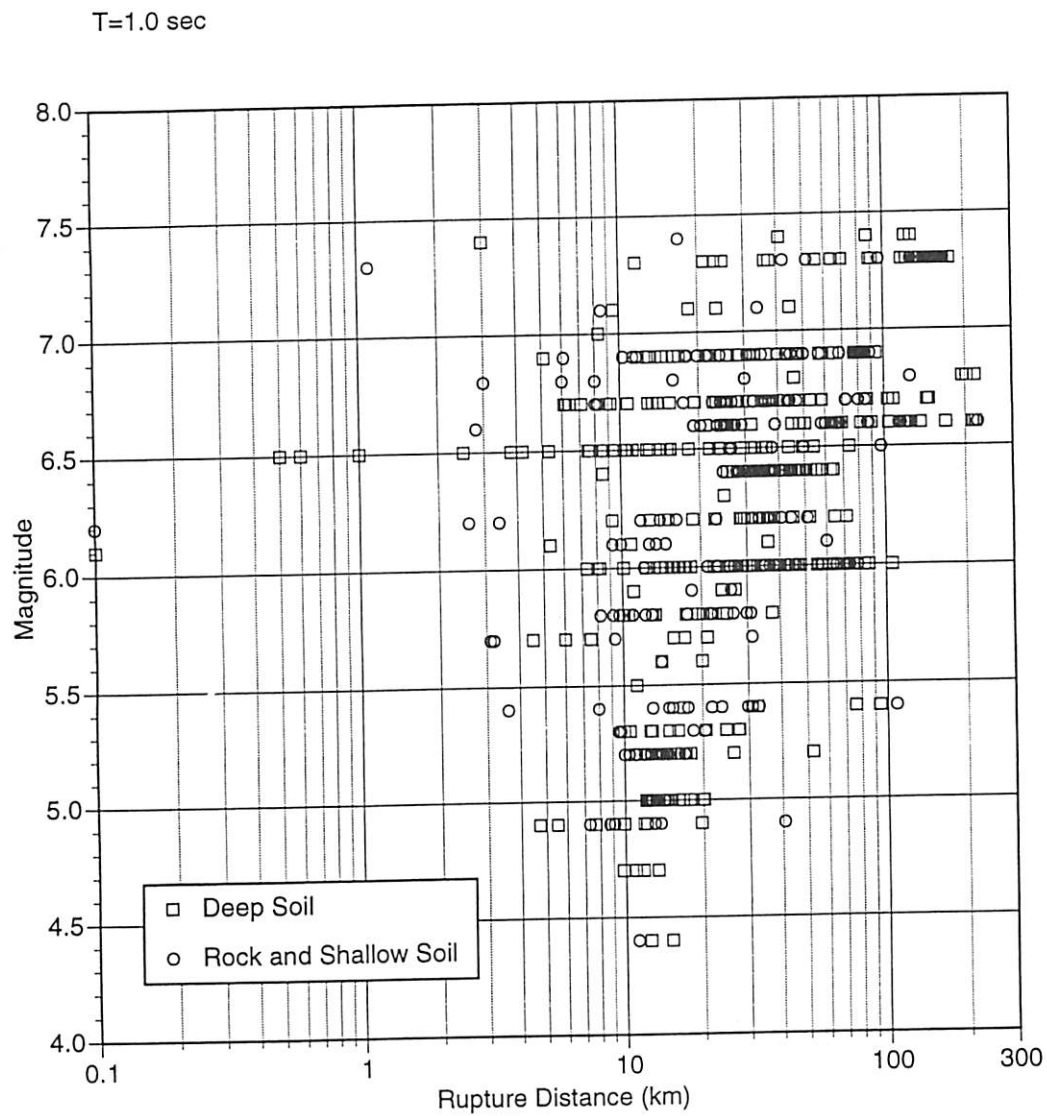
▲ Figure 2b. Distribution of data for 1.0 second period for the horizontal component.
