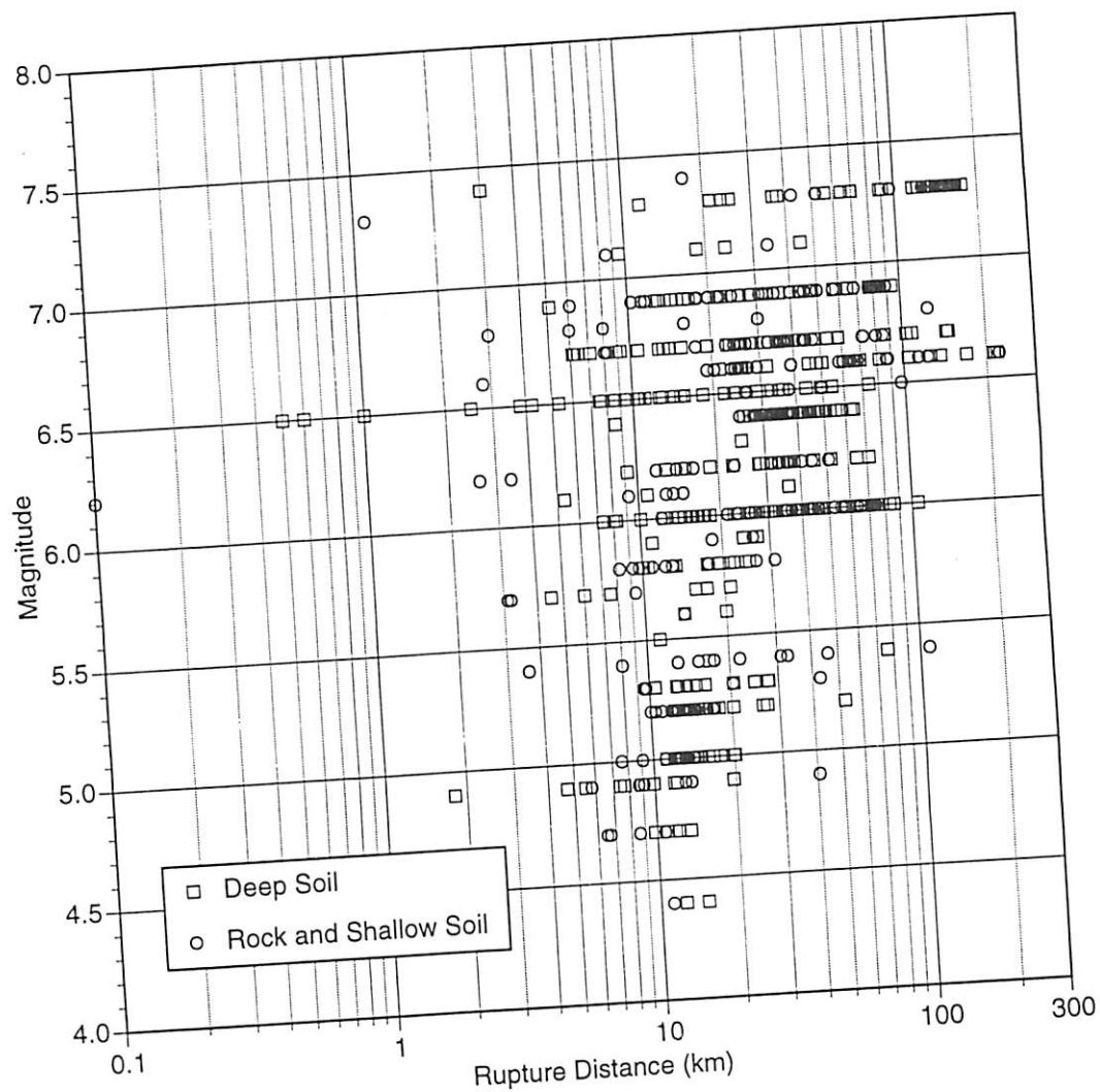
▲ Figure 2d. Distribution of data for 0.075 second period for the horizontal component.
