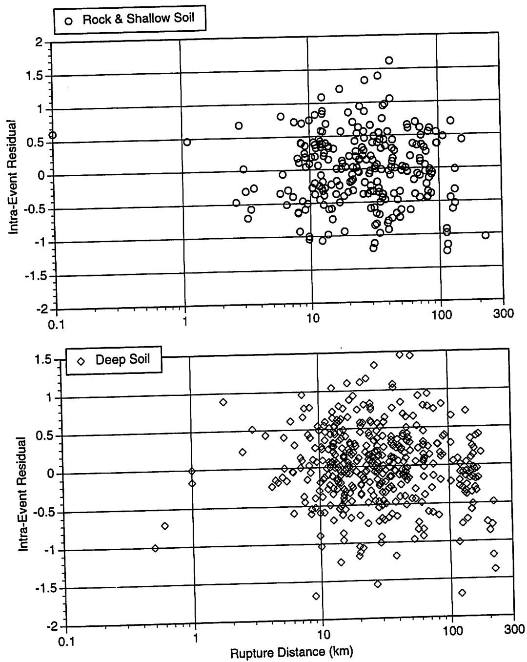
▲ Figure 4c. Distance dependence of the intra-event residuals for 0.1 second period for the horizontal component.
