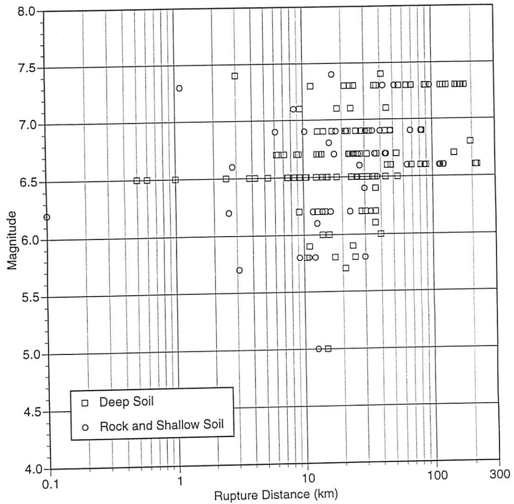
▲ Figure 3a. Distribution of data for 5.0 seconds period for the vertical component.
