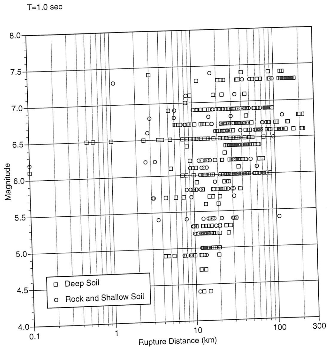
▲ Figure 3b. Distribution of data for 1.0 second period for the vertical component.
