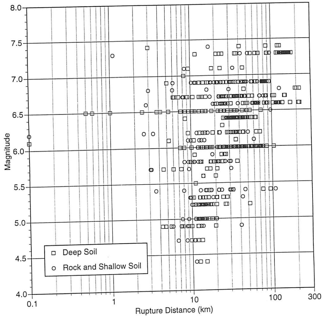
▲ Figure 3c. Distribution of data for 0.2 second period for the vertical component.
