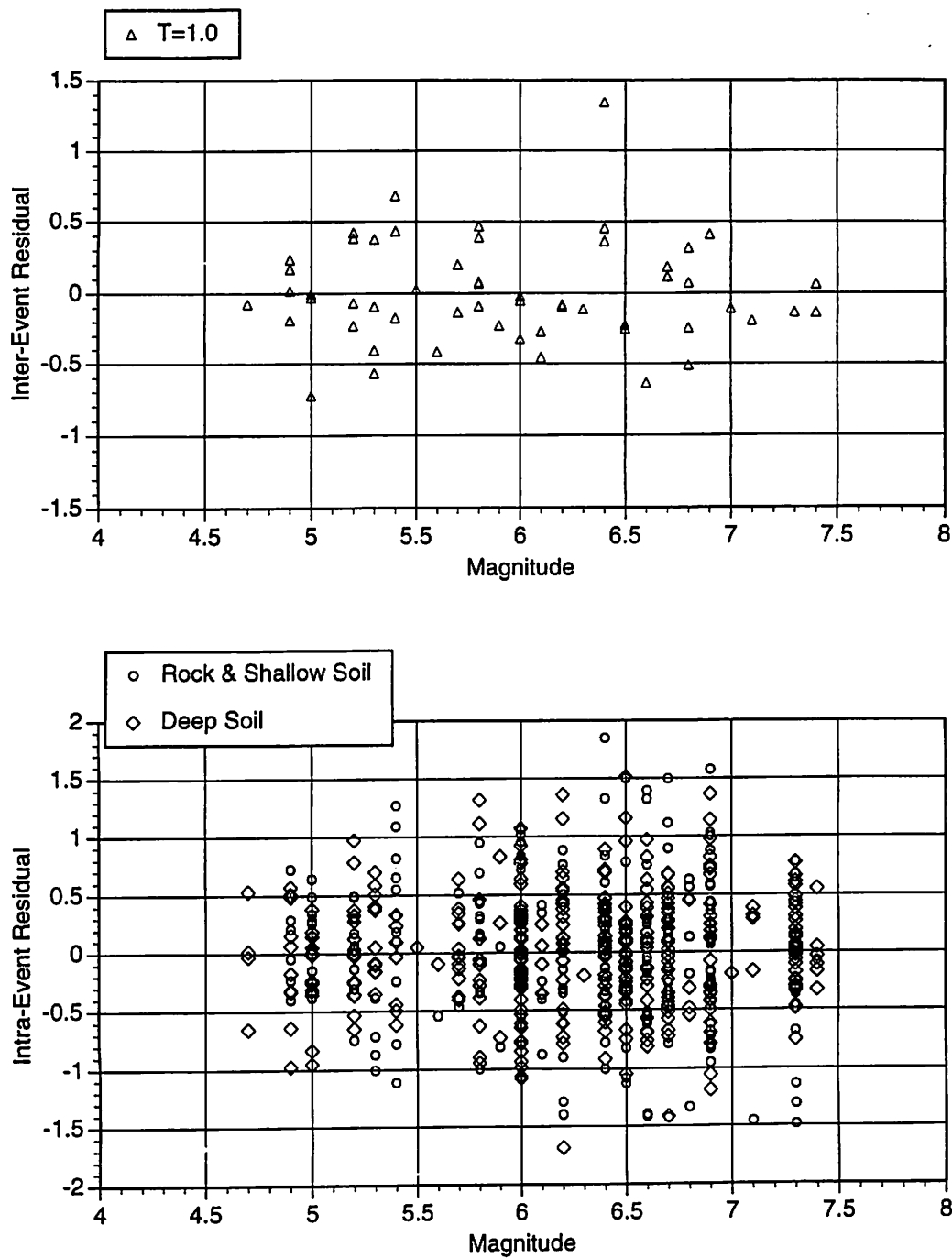
▲ Figure 5a. Magnitude dependence of the inter-event residuals (top) and the intra-event residuals (bottom) for 1.0 second period for the horizontal component.
