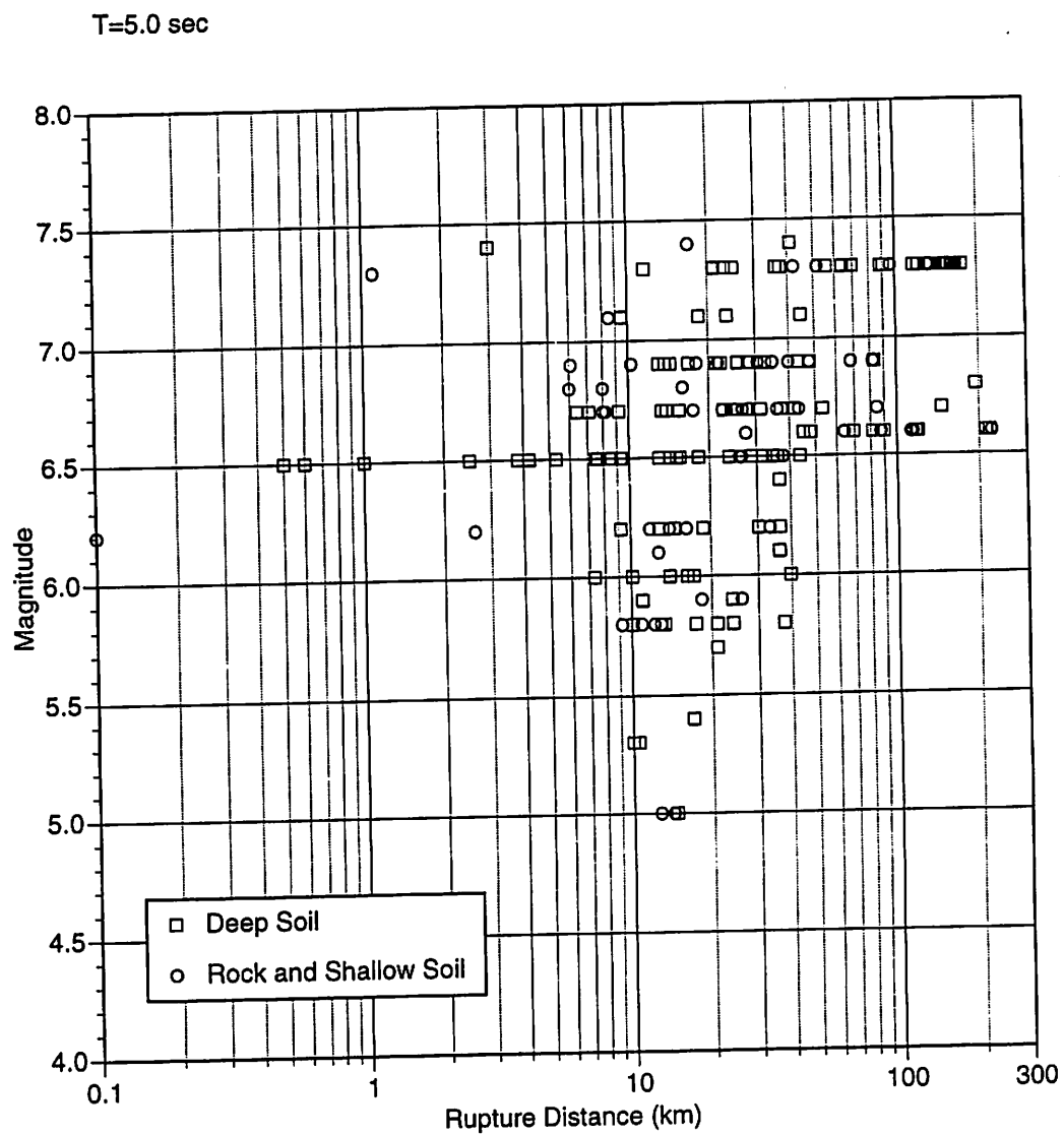
▲ Figure 2a. Distribution of data for 5.0 seconds period for the horizontal component.
