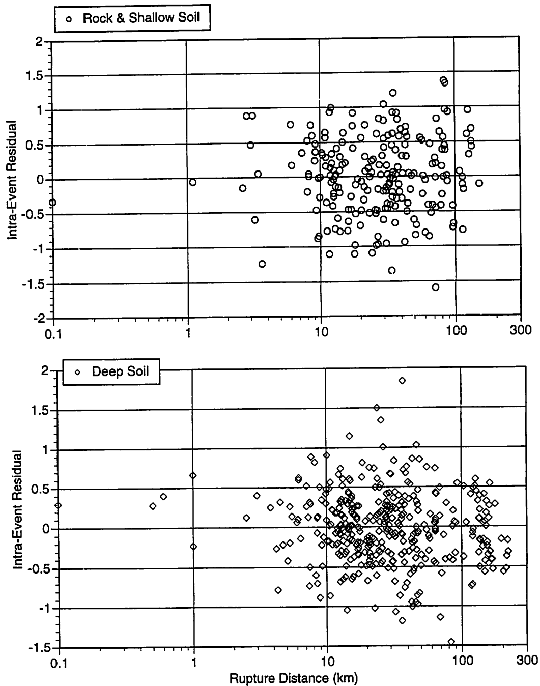
▲ Figure 6a. Distance dependence of the intra-event residuals for 1.0 second period for the vertical component.
