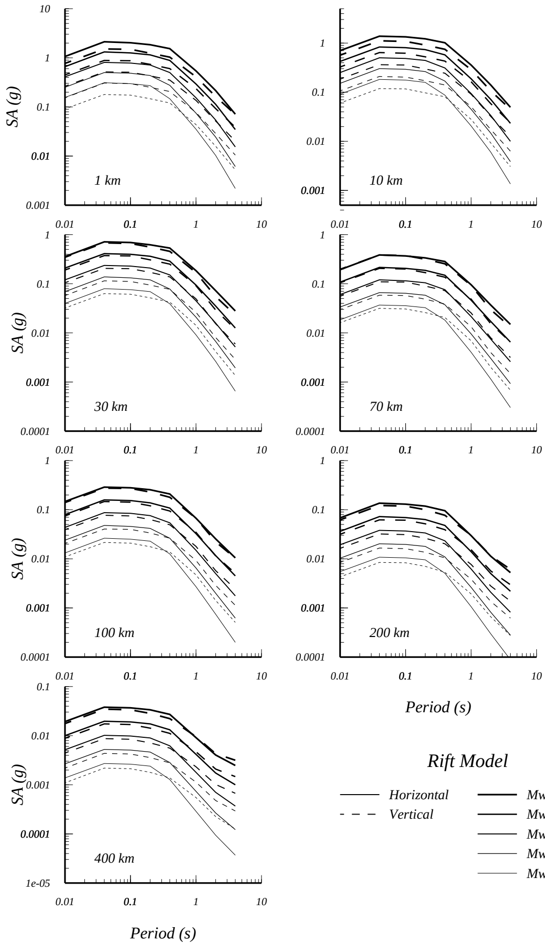
Figure 20. Rift response spectral model for a set of magnitudes and a suite of distances.
