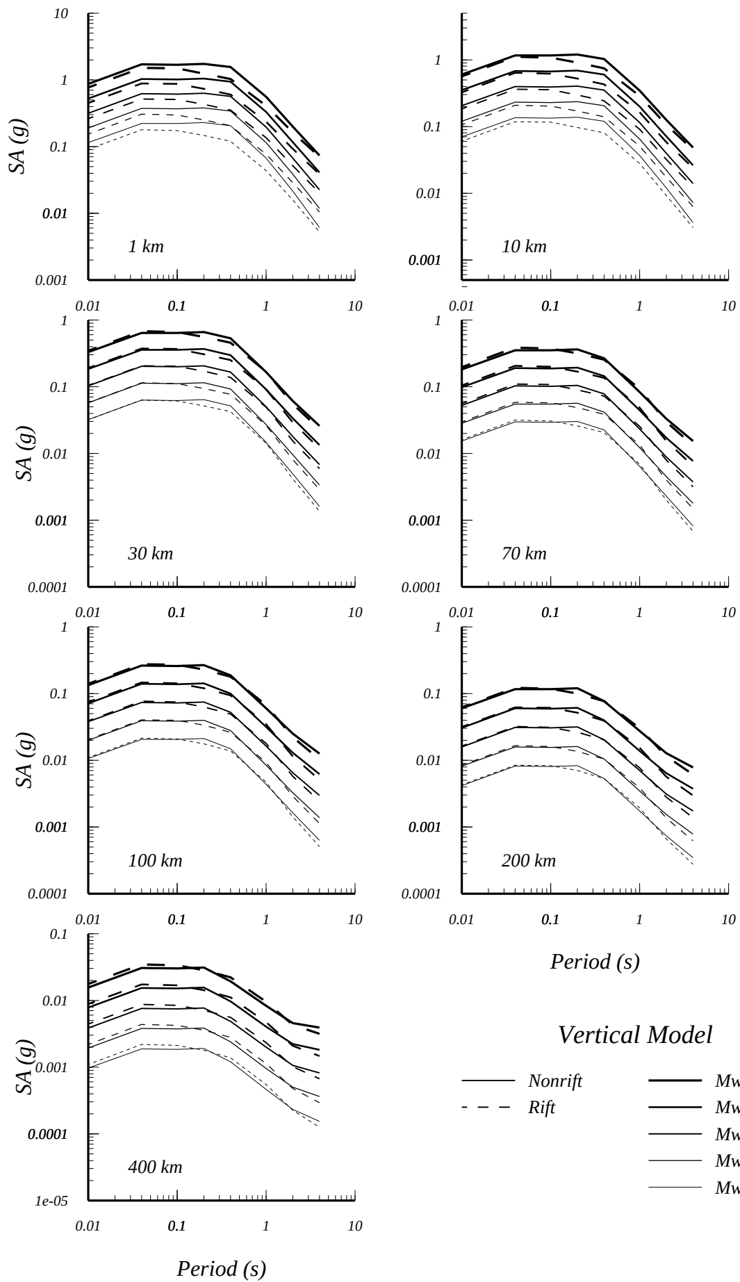
Figure 22. Vertical response spectral model for a set of magnitudes and a suite of distances.
