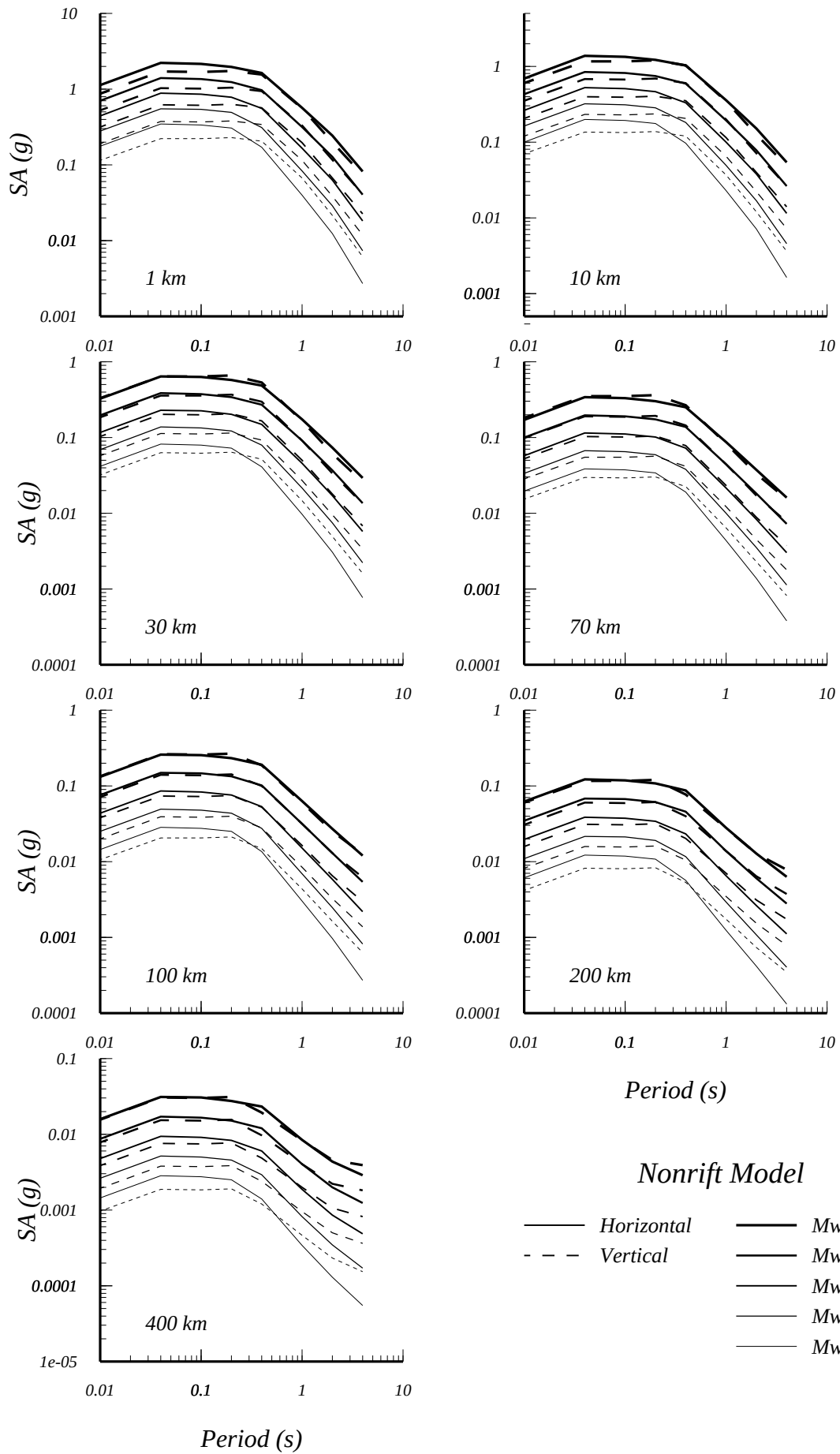
Figure 19. Nonrift response spectral model for a set of magnitudes and a suite of distances.
