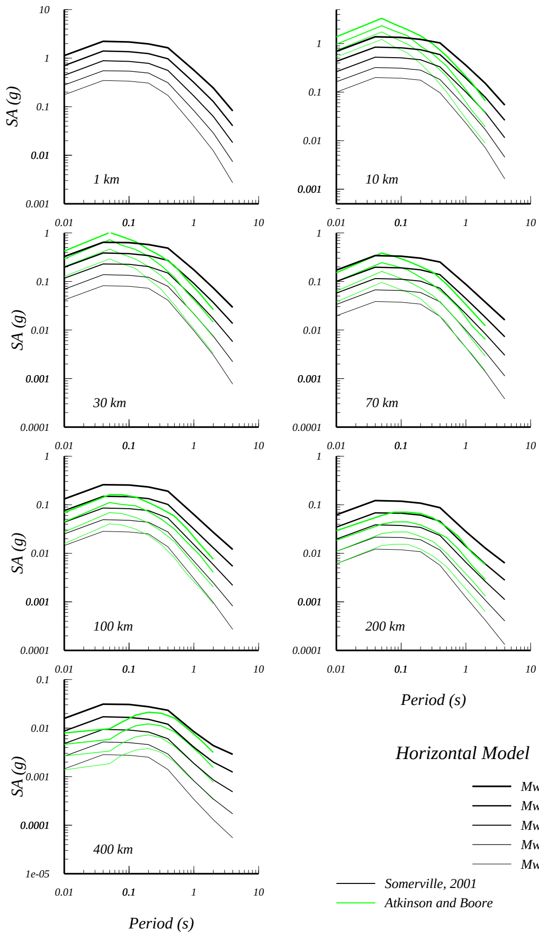
Figure 12. Non-rift model horizontal response spectral comparison with Atkinson and Boore.
