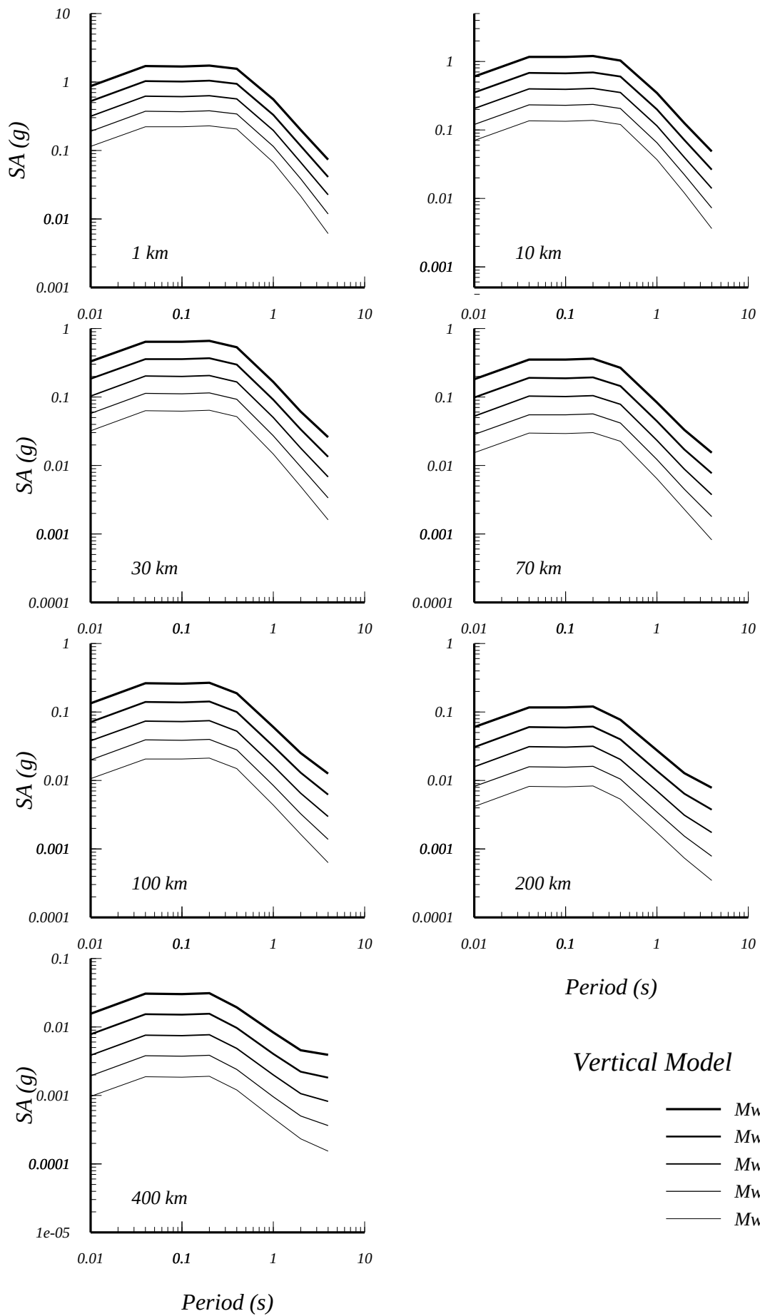
Figure 14. Non-rift model vertical response spectra.
