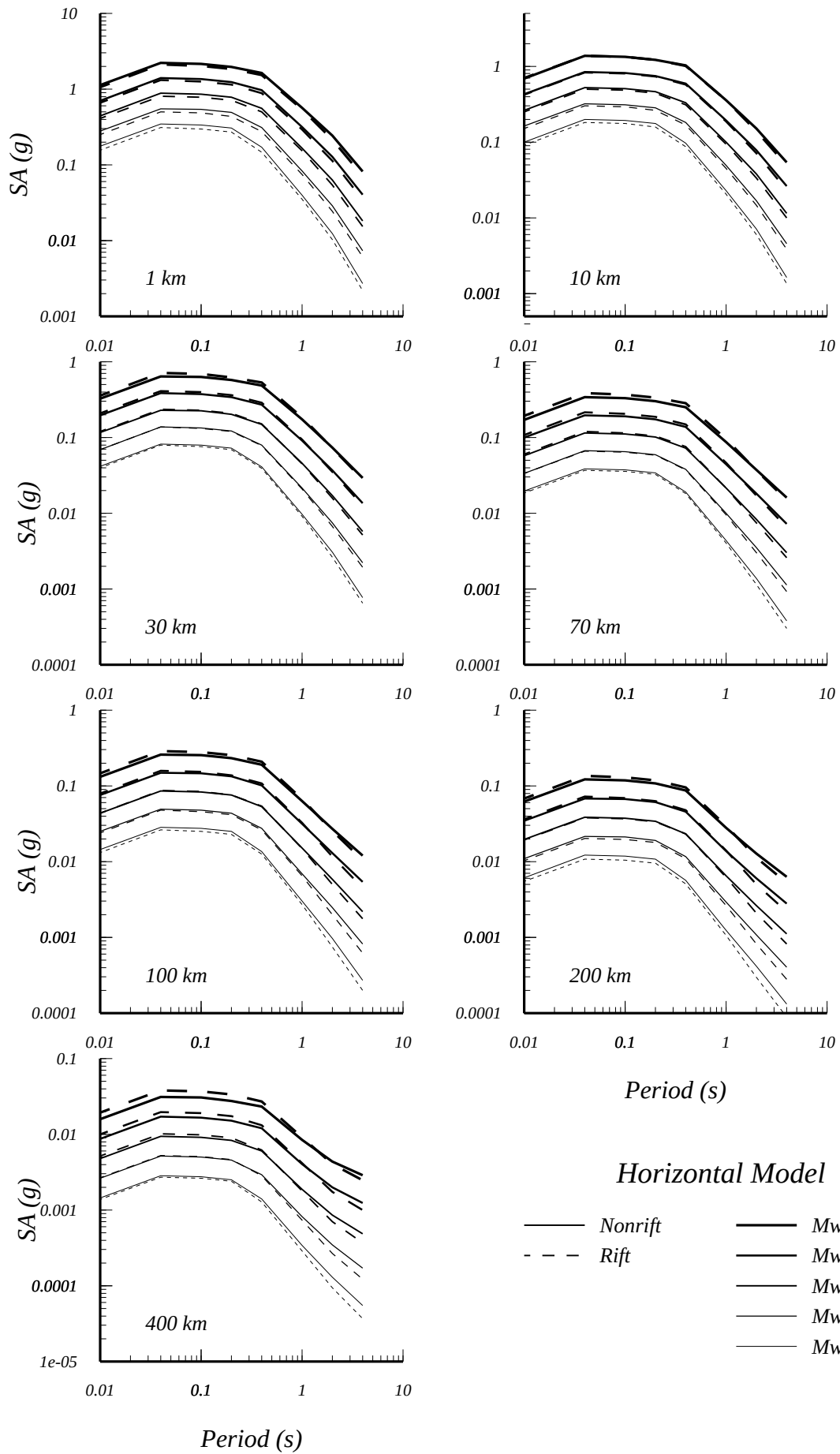
Figure 21. Horizontal response spectral model for a set of magnitudes and a suite of distances.
