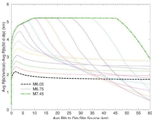
Figure D-3. Plot showing the increase in R_{jb} for vertical faults compared to 50^\circ -dipping faults as a function of average R_{jb} for the random-strike dipping fault.
