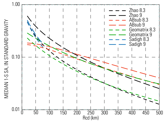
Figure 27. Plots comparing the ground-motion attenuation relations for the subduction zone interface at (A) 0.2-s and (B) 1-s spectral acceleration (SA) at firm-rock site based on Zhao 8.3 and Zhao 9, Zhao and others (2006); ASub 8.3 and ASub 9, Atkinson and Boore (); Geomatrix 8.3 and Geomatrix 9, Geomatrix Consultants, Inc. (1995); Sadigh 8.3 and Sadigh 9, Sadigh and others (1997).
