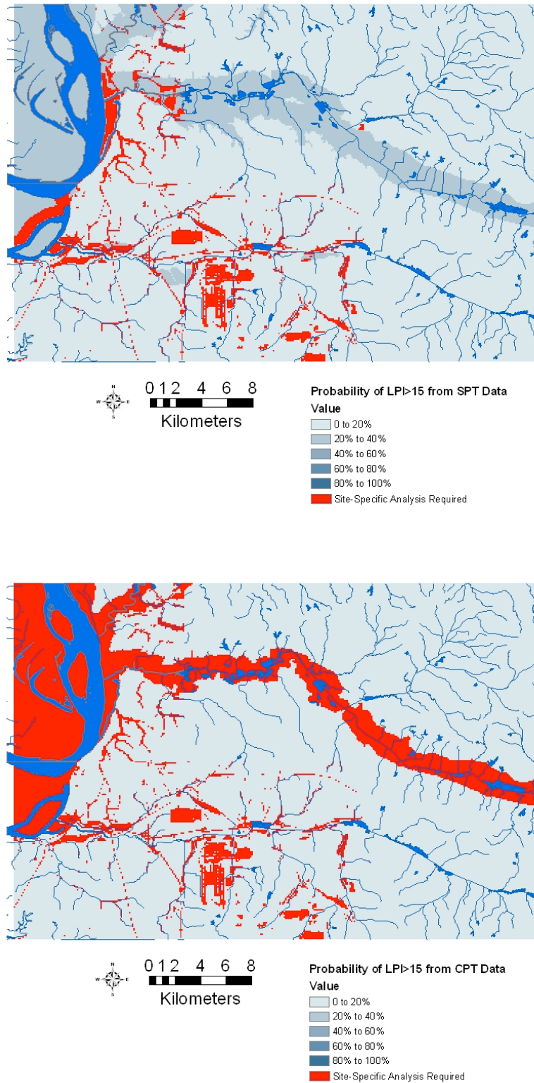
Figure 10. Probability of Major Liquefaction ( LPI > 15 ) in the Study Area due to a M_w = 7.7 Scenario Earthquake from (a) SPT and (b) CPT data
