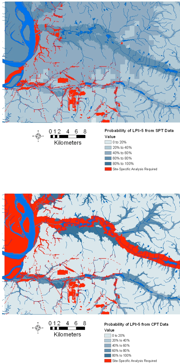
Figure 9. Probability of Moderate Liquefaction ( LPI > 5 ) in the Study Area due to a M_w = 7.7 Scenario Earthquake from (a) SPT and (b) CPT data
