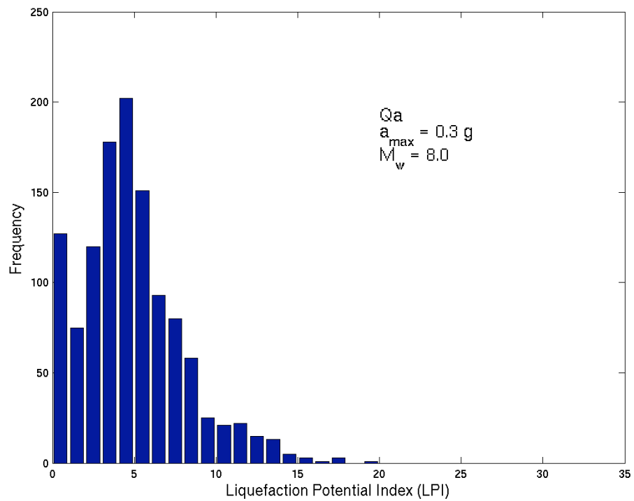
Figure 4. Histogram of LPI for (a) SPT data and (b) CPT data for Unit Qa, a_{\max} = 0.3 \text{ g} , and M_w = 8.0
