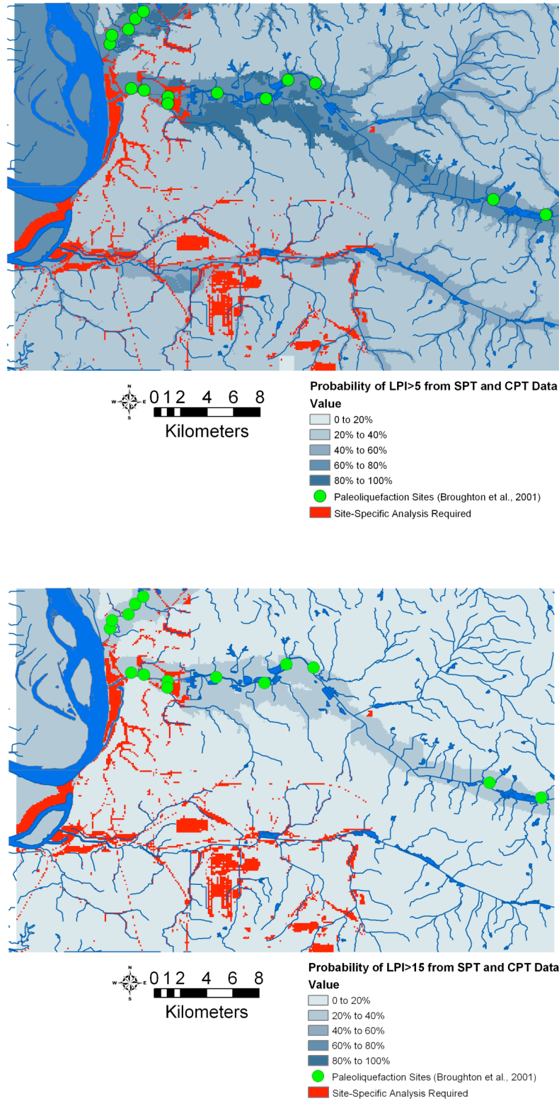
Figure 11. Probability of (a) Moderate ( LPI > 5 ) and (b) Major ( LPI > 15 ) Liquefaction in the Study Area due to a M_w = 7.7 Scenario Earthquake from Combined SPT and CPT data and Comparison with Paleoliquefaction Features
