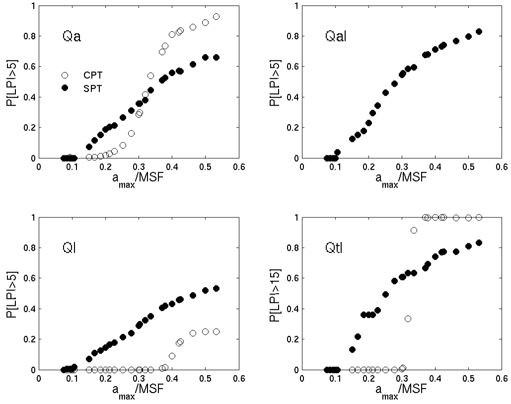
Figure 5. Probability of LPI > 5 for each Geologic Unit
