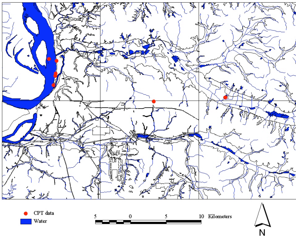
Figure 2. Location of (a) SPT and (b) CPT profiles
