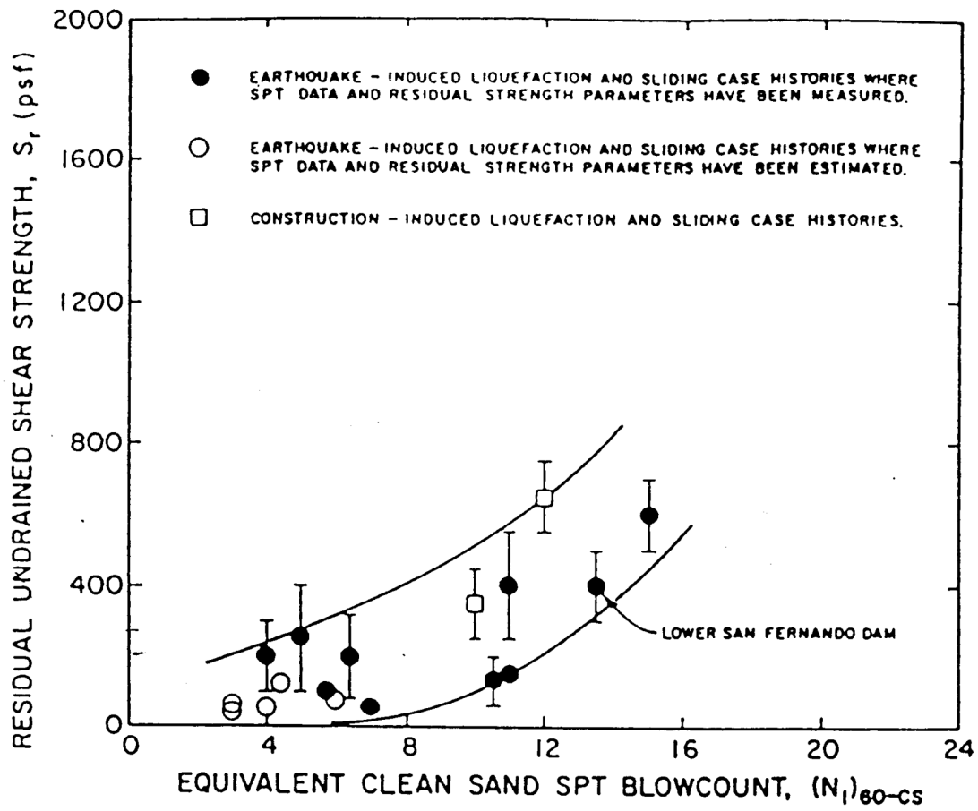
RECOMMENDED FINES CORRECTION FOR S_r EVALUATION USING SPT DATA
