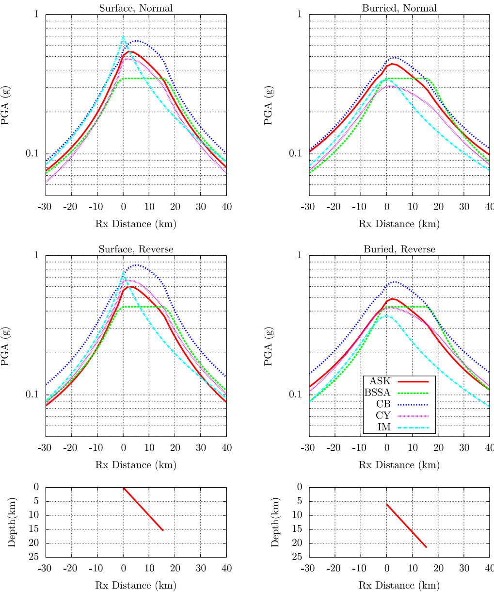
Figure 6. Comparison of FW and HW effects on PGA for a 45-degree, M 6.7 earthquake for V_{S30} = 760 m/s for both surface rupture (left side) and buried rupture (right side) with a top-of-rupture of 6 km.
