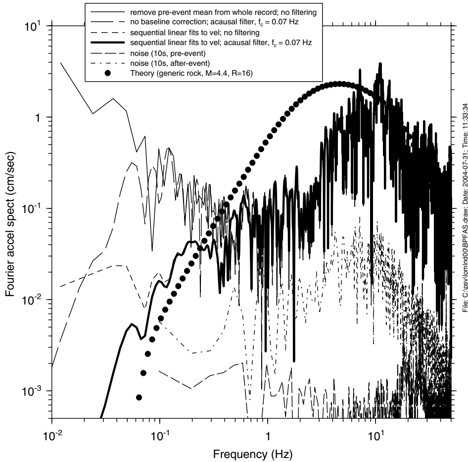
Fig. 6. The Fourier acceleration spectra for the acceleration time series from which the velocities and the displacements shown in the previous two figures were derived, along with the spectra of 2 10-sec noise samples (pre-event and near the end of the record). Also shown is the theoretical spectrum, including low-cut filtering with a 0.07 Hz low-cut filter. Clearly, making the multisegment baseline correction buys a lot (compare the short-dashed line and light solid line)—it seems that we can obtain reasonable results to 0.1 Hz, where “reasonable” is a subjective judgement based on the appearance of the spectra. The “noise” introduced by the baseline offsets is sufficient that simple filtering by itself is not adequate for this record (this “noise” is not the same as the pre- and post-event noise whose spectra are shown here; that noise is much less important than the “signal-generated noise” produced by the baseline offsets).
