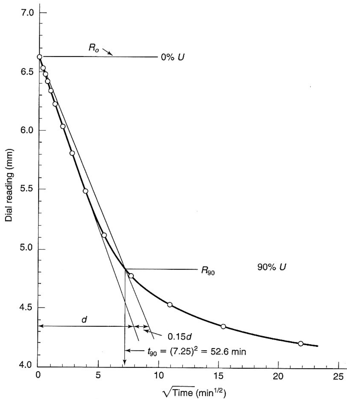
FIGURE 9.14 Determination of c_{vr} using Taylor's square root of time method; data from Table 9.2.
